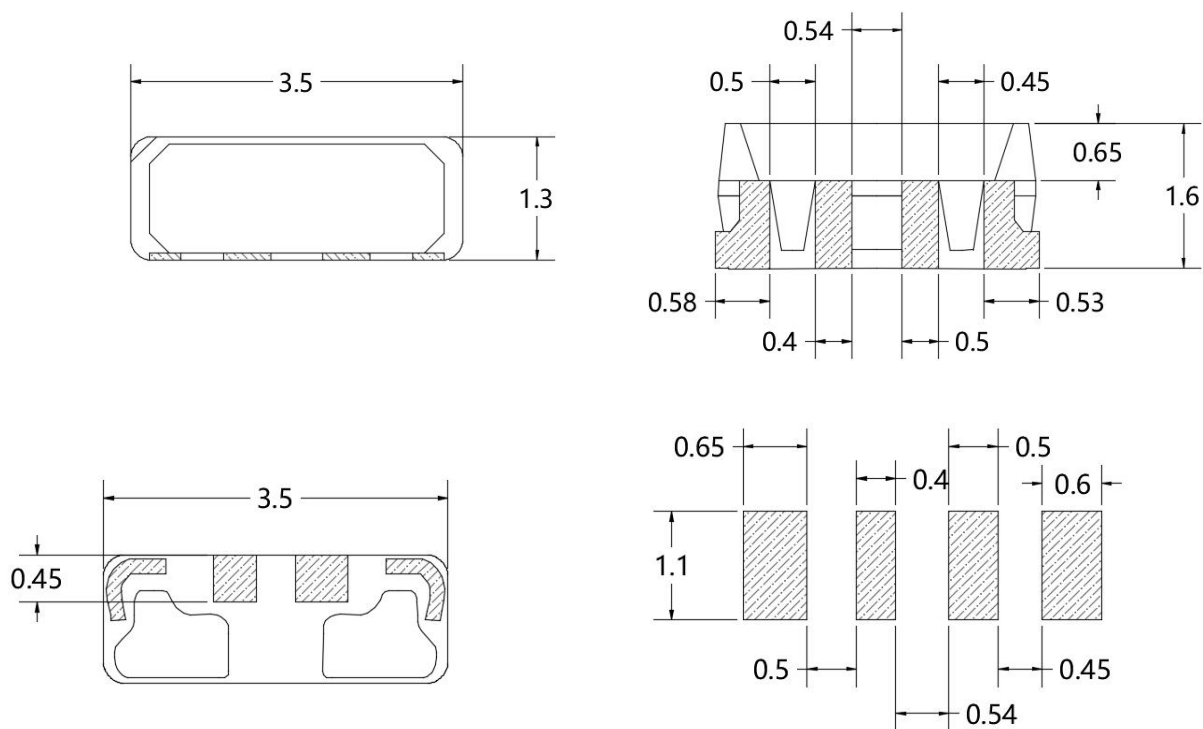
建议焊盘尺寸 Recommended Soldering Pattern
