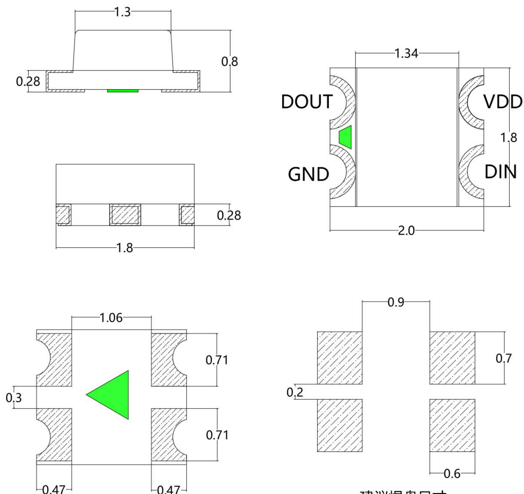
建议焊盘尺寸 Recommended Soldering Pattern
