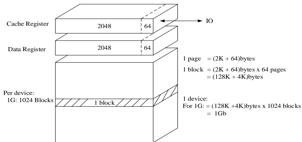
Figure 3. Array Organization
