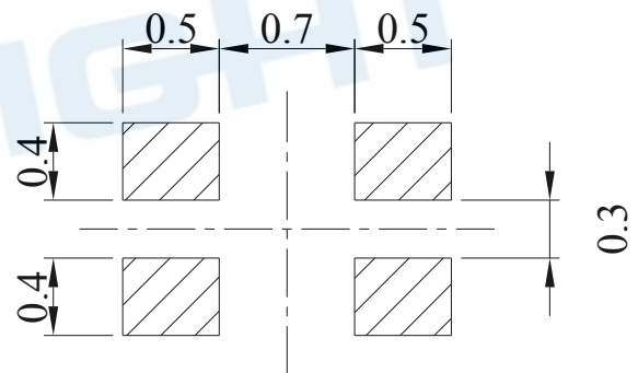
Recommend Soldering Pad
