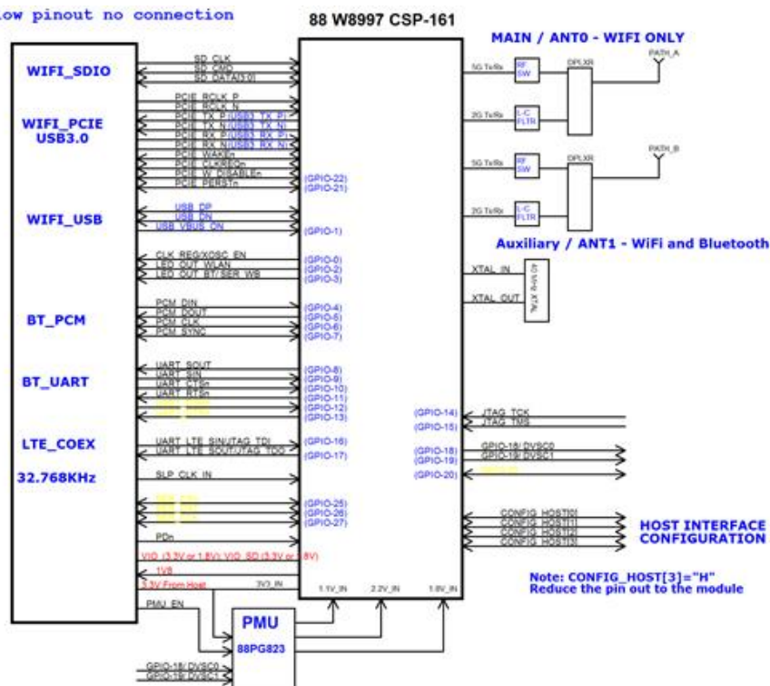
Figure 1: Block diagram
