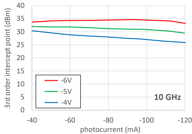
Fig. 3: Output IP3 versus photocurrent.
