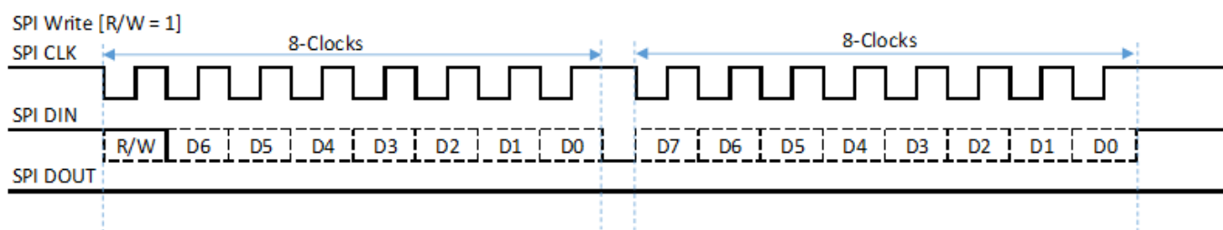
Figure 4: SPI Write Timing Diagram
