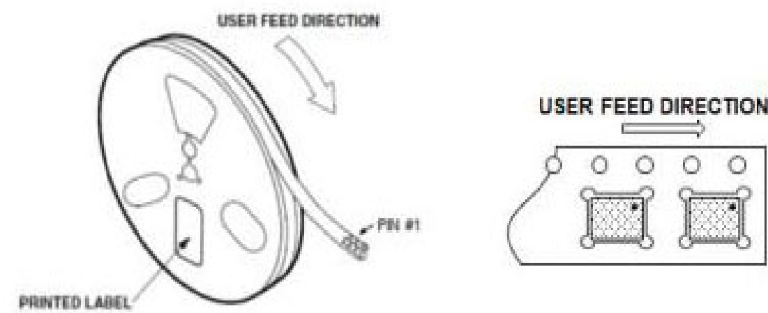
Figure 14: Reel Orientation
