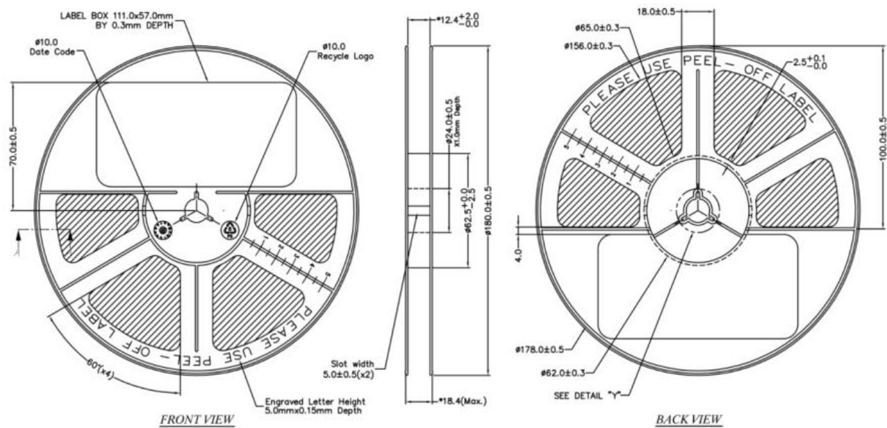
Figure 13: Tape Dimensions
