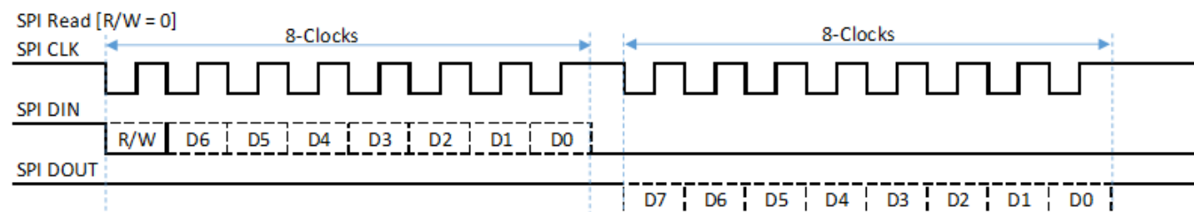
Figure 5: SPI Read Timing Diagram
