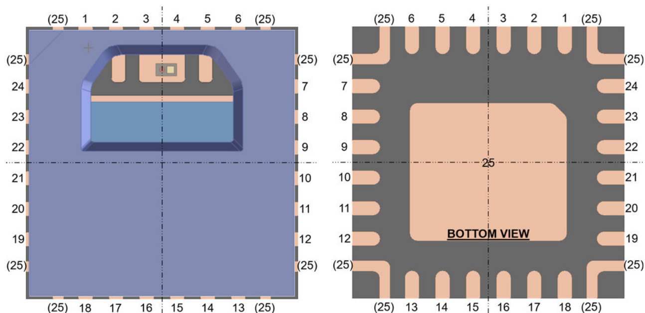
Figure 2: Encoder Pinout
