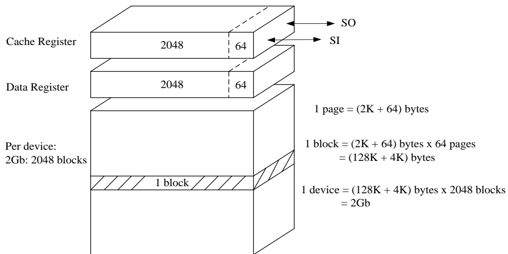
Figure 3-1. Array Organization
