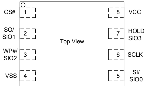
8 - LEAD WSON
