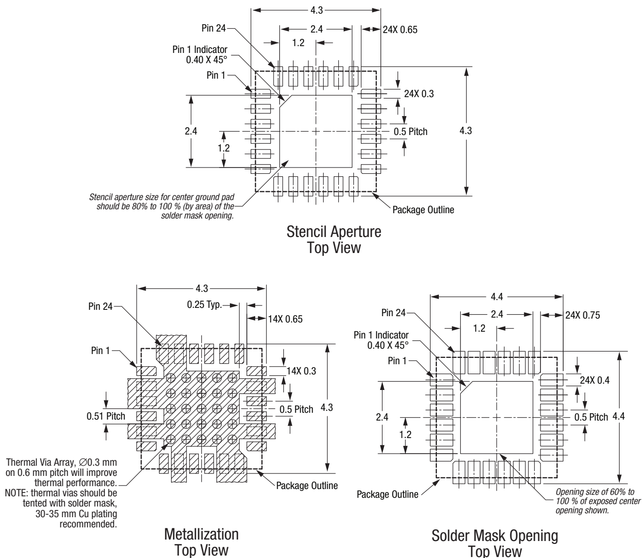
Figure 7. SE5516A PCB Layout Footprint
