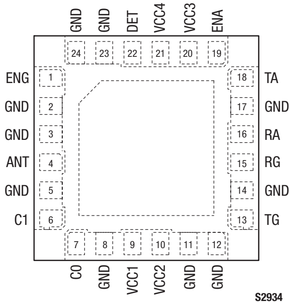
Figure 2. SE5516A Pinout (Top View)
