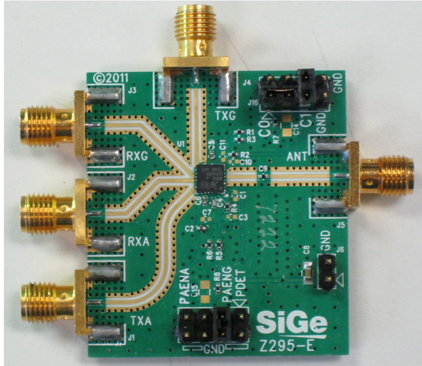
Figure 6. SE5516A Evaluation Board Photo
