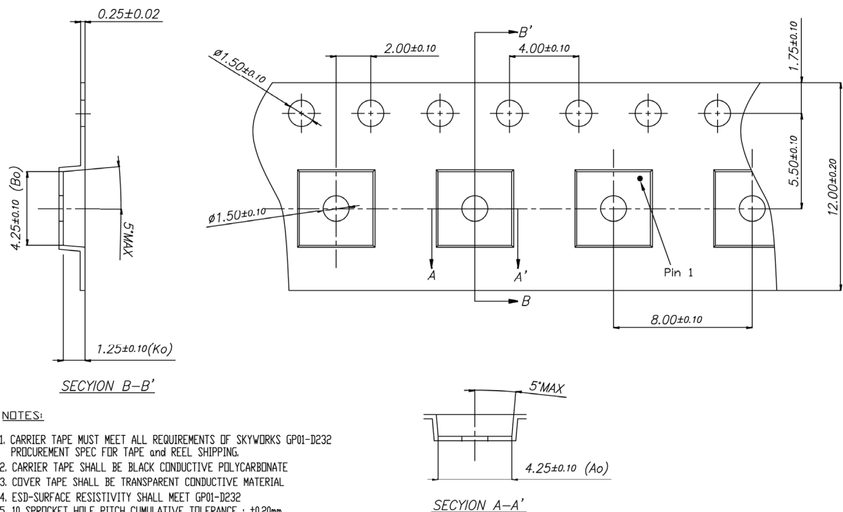
Figure 10. SE5516A Tape and Reel Dimensions
