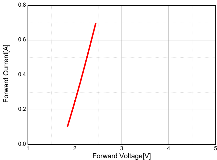
Forward Voltage vs. Forward Current, T_a=25^\circ\text{C}
