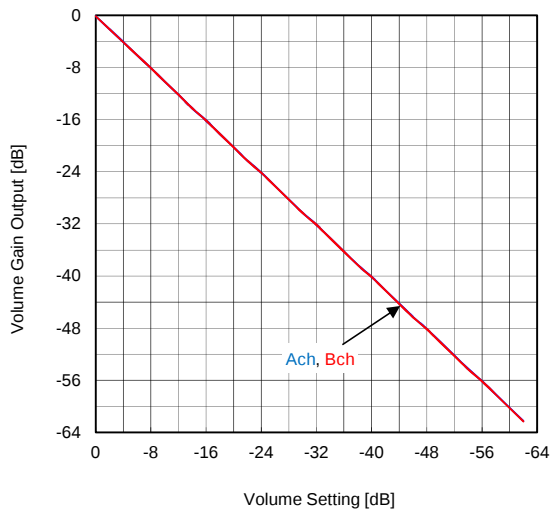
Volume Gain Output vs Volume Setting V=\pm 5V , f=1kHz , V_{in}=2V_{rms} , Bandpass
