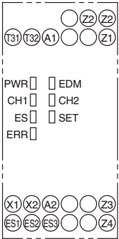
Terminal arrangement
