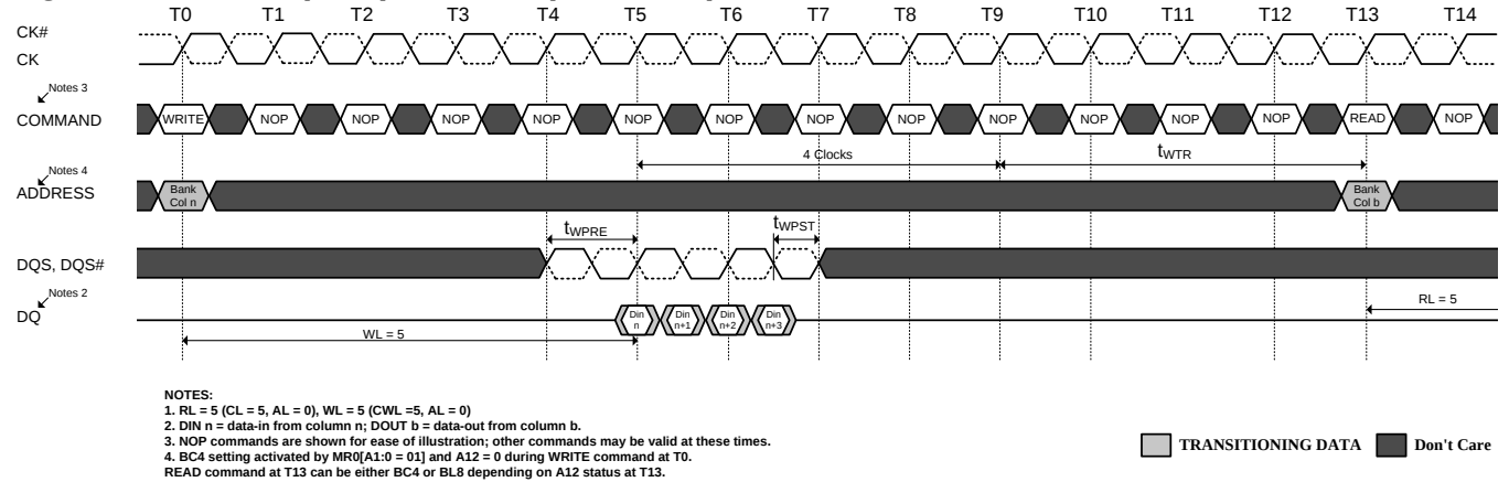
Figure 51. WRITE(BC4) to READ(BC4,BC8) OTF
