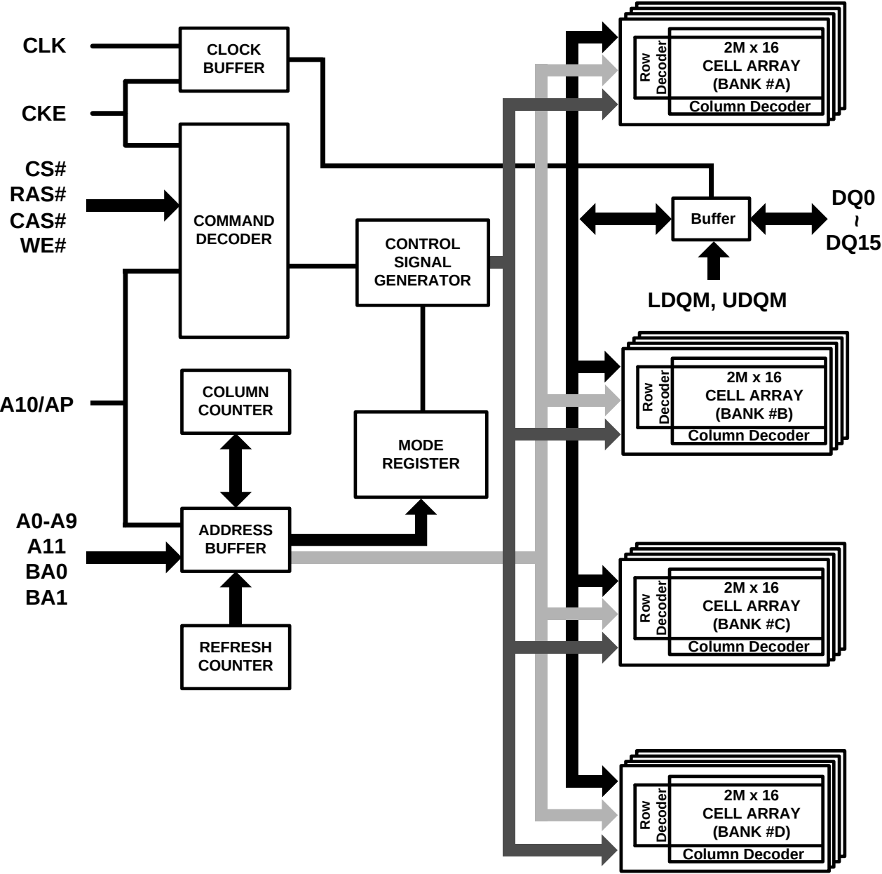
Figure 2. Block Diagram
