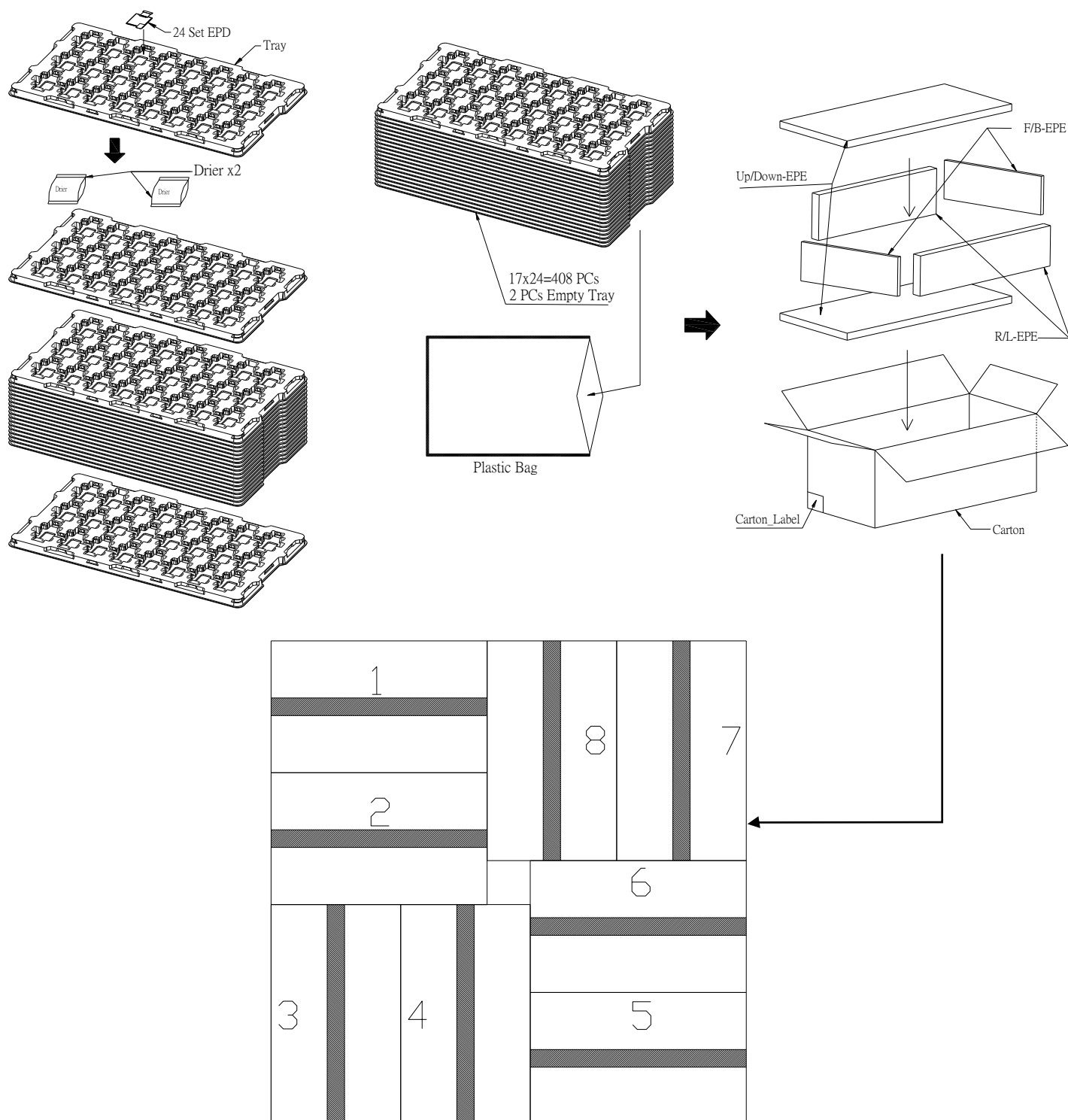
Figure 7-1 Packing Diagram
