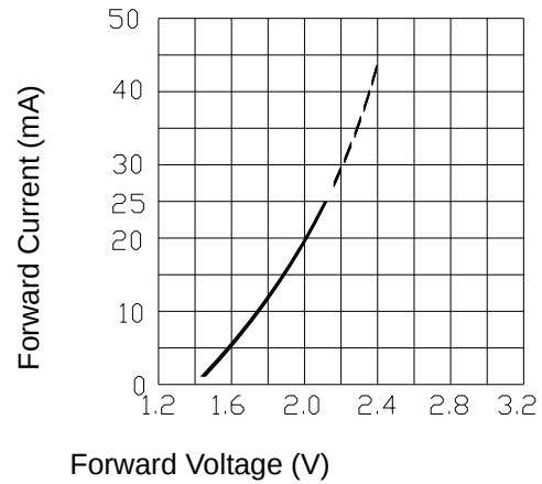
Forward Current vs. Forward Voltage (Ta=25°C)
