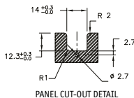
Panel mounting details
