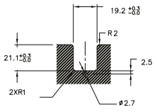
Panel mounting details
