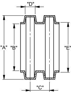
Fig. 1 Solid Version
