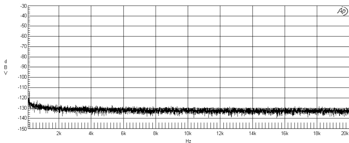
Noise spectrum at Vdd = 5.0Vdc, Gain = 0dB, BW<22kHz
