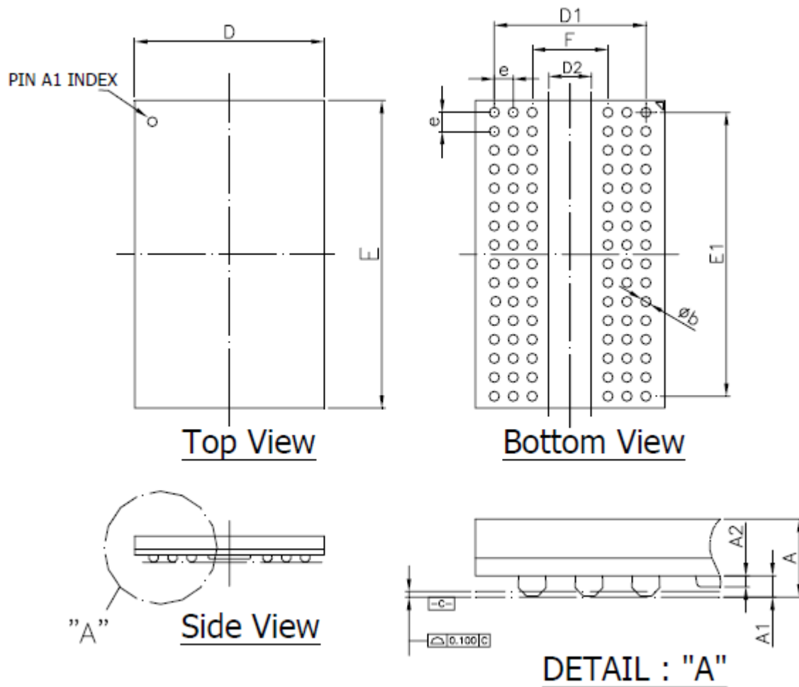
Figure 82. 96-Ball FBGA Package 8x13x1.0mm(max) Outline Drawing Information
