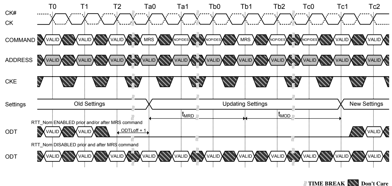
Figure 6. t_{MRD} timing
