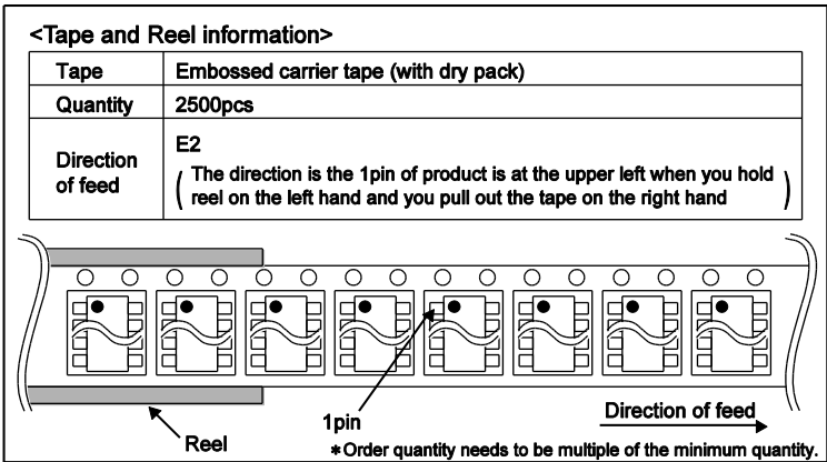
Figure 20. Tape and reel information
