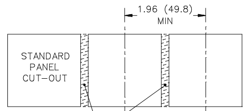
PANEL CUT-OUT SPACING FOR MULTIPLE UNIT STACKING. HORIZONTAL ARRANGEMENT SHOWN.
