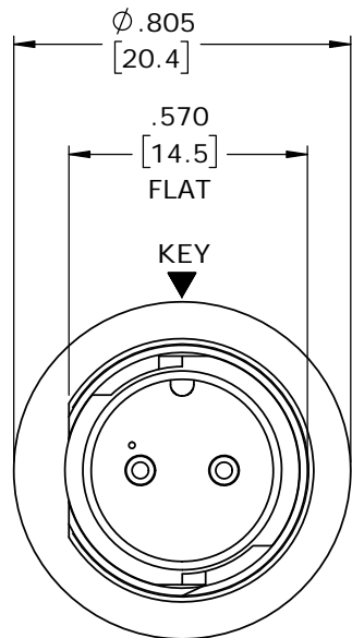
MATING FACE W7282-2PG-P-300 SHOWN
