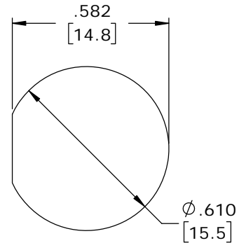
RECOMMENDED PANEL CUTOUT TOLERANCE ±.003 [.08]
