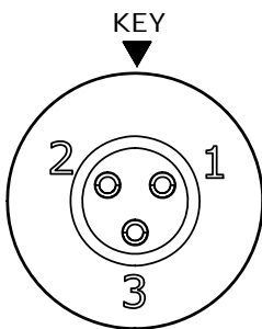
WIRING END W7282-3PG-P-300
