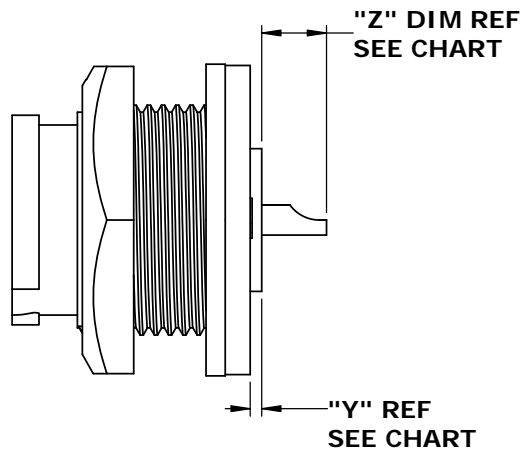
ASSEMBLED VIEW W7282-2PG-P-300 SHOWN
