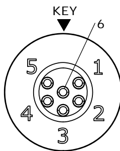
WIRING END W7282-6PG-P-300
