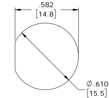
RECOMMENDED PANEL CUTOUT TOLERANCE ±.003 [0.08]
