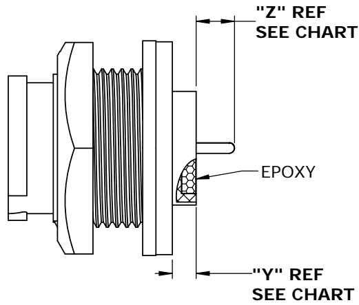
ASSEMBLED VIEW W7281-2SG-P-3ES SHOWN
