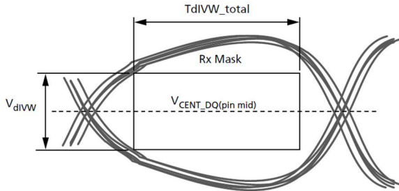
Figure 27 - DQ Receiver (Rx) Mask
