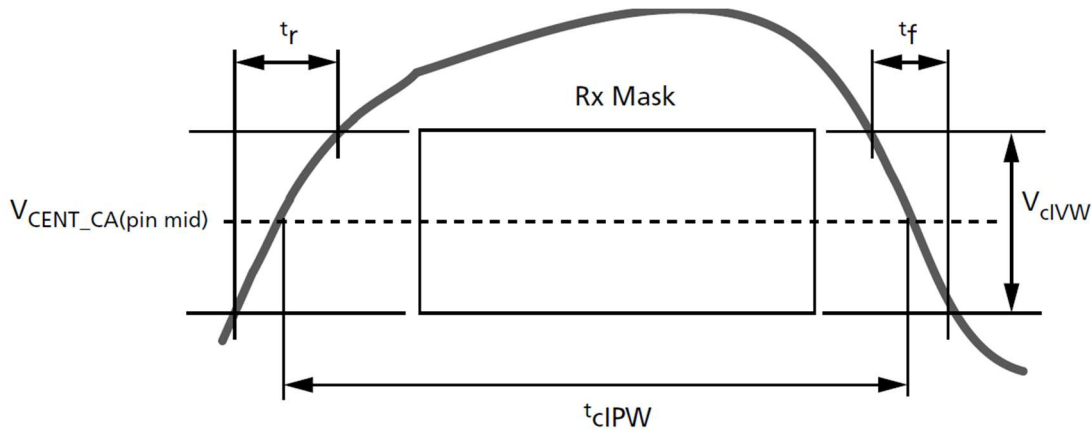
Figure 23 - CA tClPW and SRIN_cIVW Definition (for Each Input pulse)
