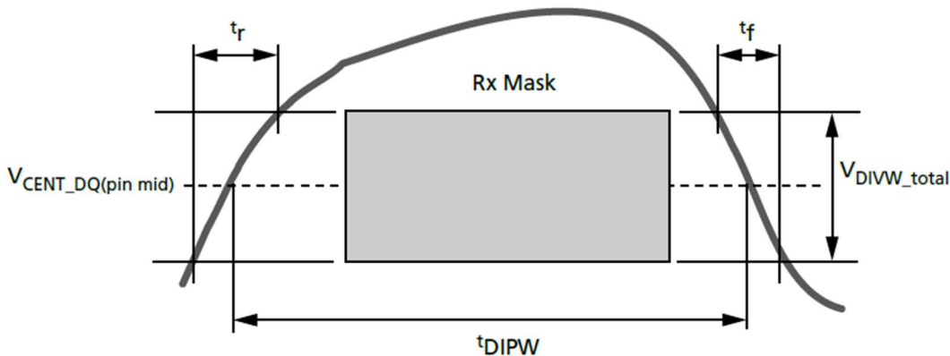
Figure 29 - DQ t_{DIPW} and SRIN\_dIPW Definition for Each Input Pulse
