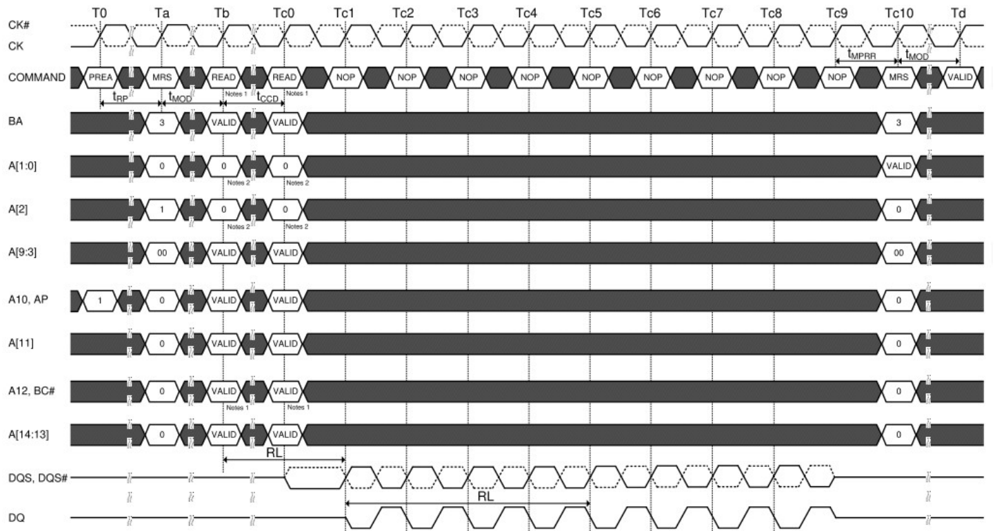
Figure 21 - MPR Readout of predefined pattern, BL8 fixed burst order, back to back readout
