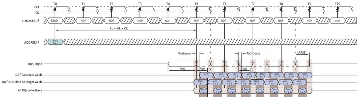
Figure 28 - Data Strobe to Data Relationship
