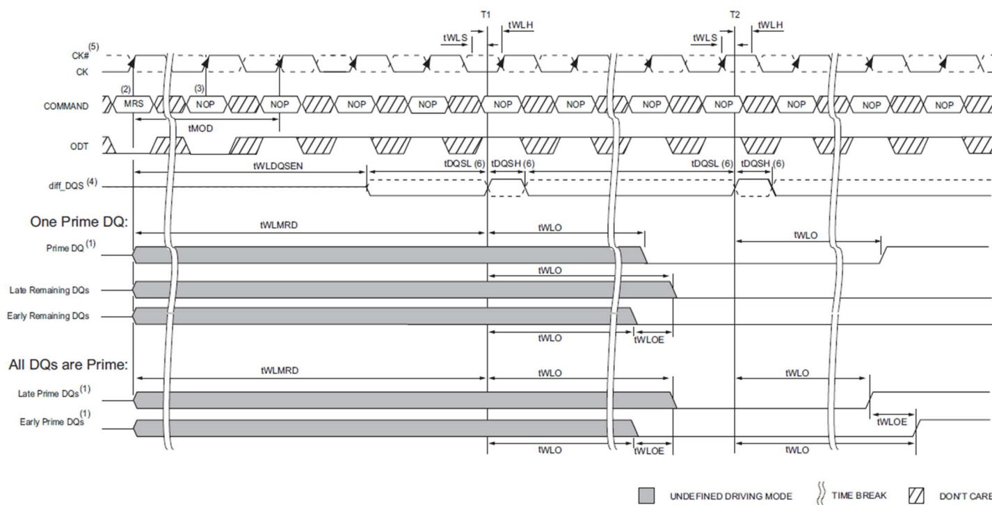
Figure 17 - Timing detail for Write leveling sequence [DQS-DQS# is capturing CK-CK# low at T1 and CK-CK# high at T2]
