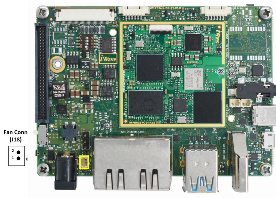
Figure 26: Fan Connector
