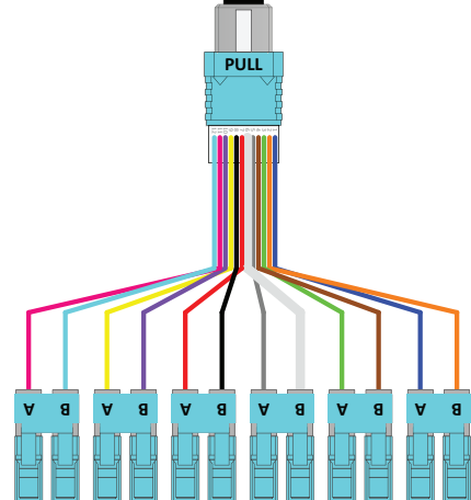
FX Hydra Assembly Type A Polarity MPO-12 12 Fiber
