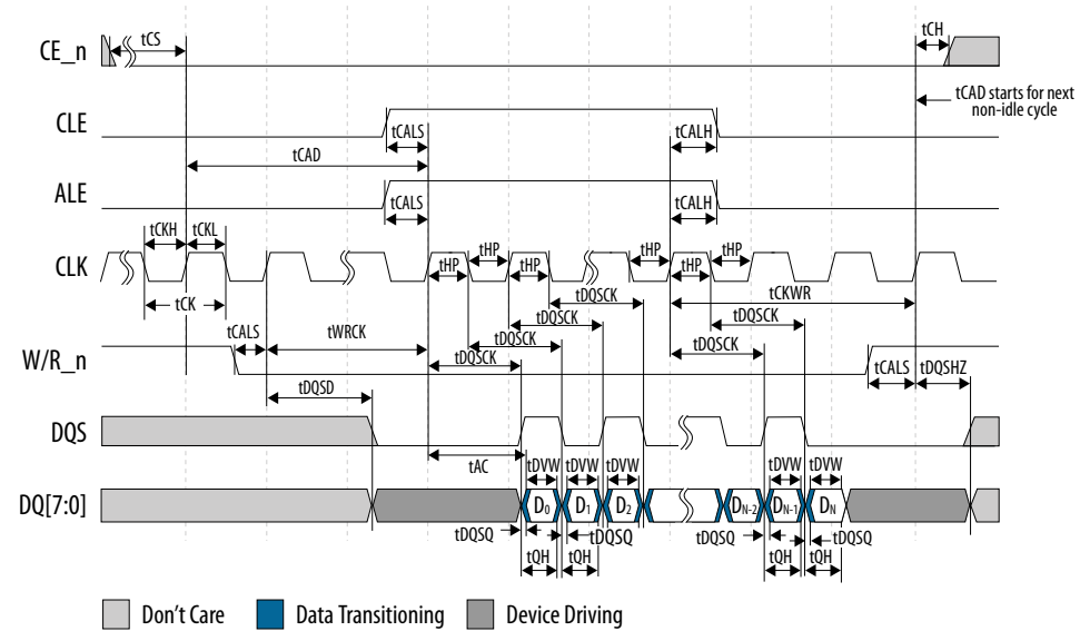
Figure 42. NAND DDR Data Output Cycle Timing Diagram
