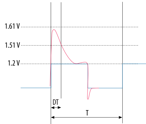
Figure 1. Overshoot Duration Example (for 1.2 V HSIO Bank at V_{\text{CCIO\_PIO}} = 1.26 \text{ V} )
