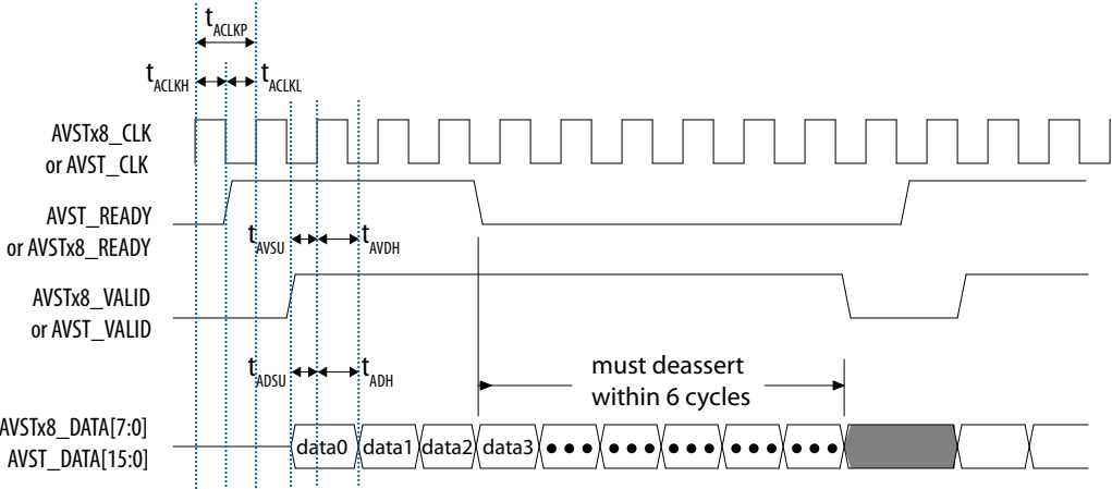
Figure 51. Avalon Streaming Configuration Timing Diagram
