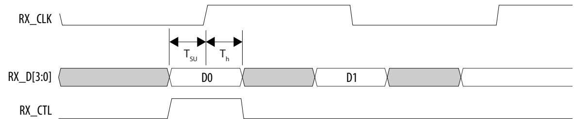
Figure 20. RGMII RX Timing Diagram
