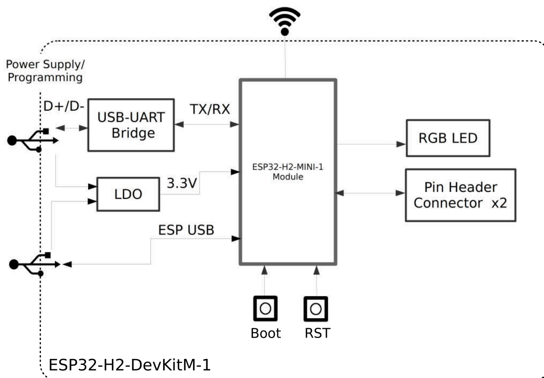
Fig. 3: ESP32-H2-DevKitM-1
