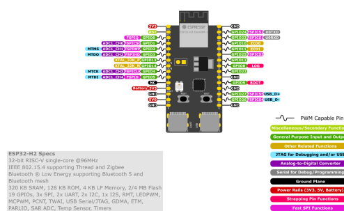
Fig. 4: ESP32-H2-DevKitM-1 Pin Layout
