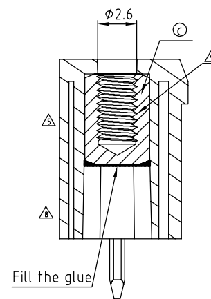
SECTION P-P
