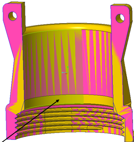
New and existing part overlay
