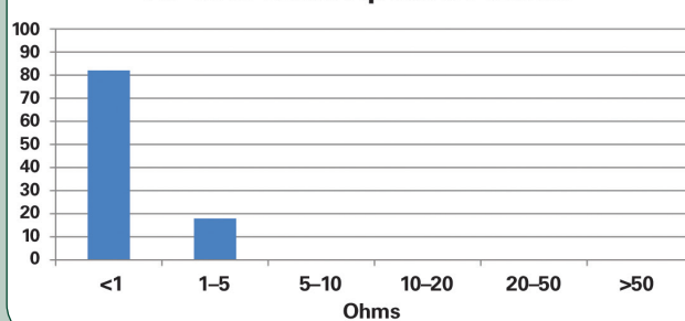
WF-9940 Chisel Tip SnPb Process
