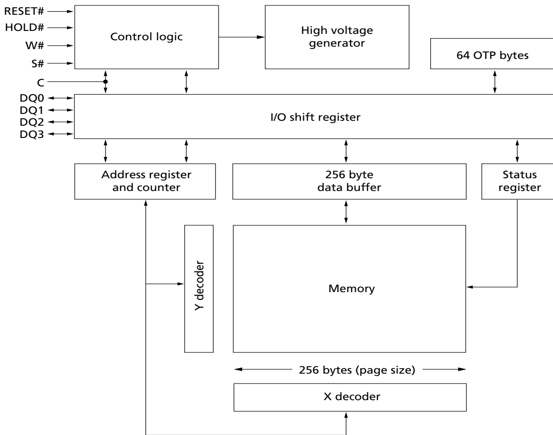
Figure 2: Block Diagram
