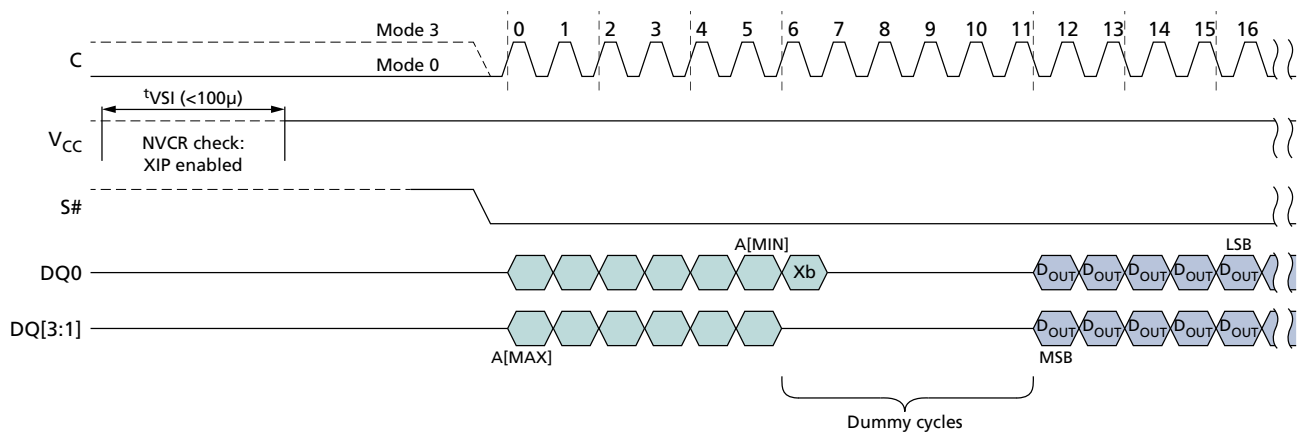
Figure 38: XIP Mode Directly After Power-On
