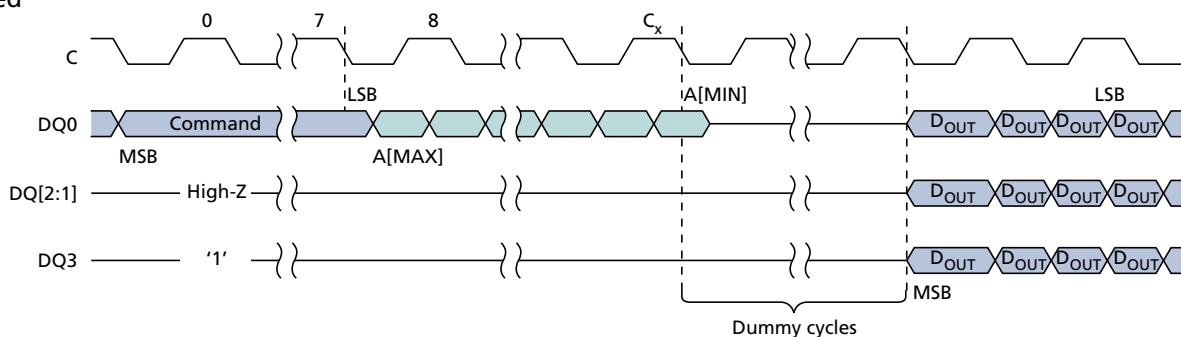
Figure 21: DTR QUAD OUTPUT FAST READ – 6Dh 3
