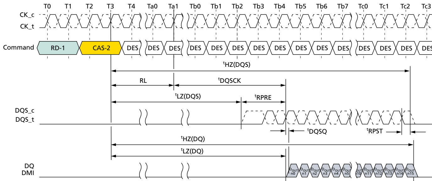
Figure 24: Read Timing
