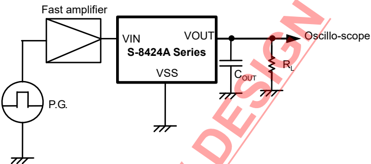
Figure 14 Test Circuit
