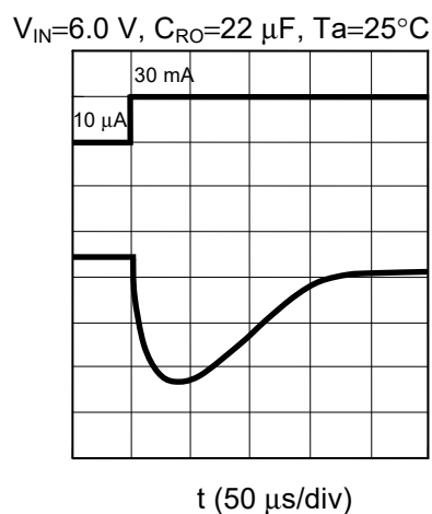
Figure 20 Ringing Waveform due to Load Variation (VRO Pin)
