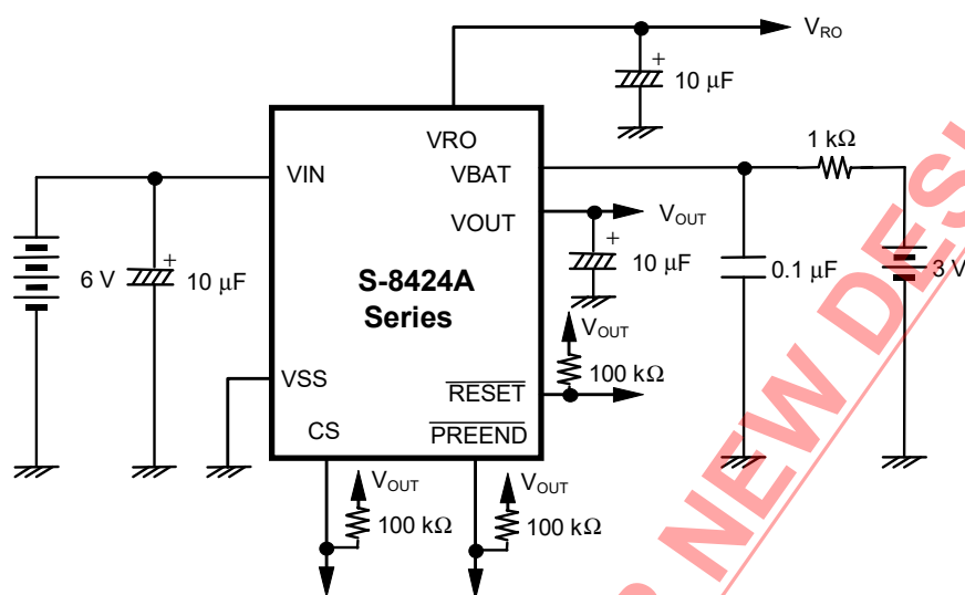
Figure 21 Standard Circuit
