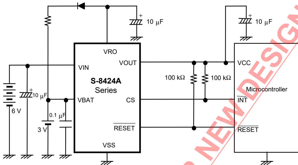
Figure 23 Application Circuit 2
