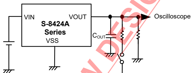
Figure 18 Test Circuit
