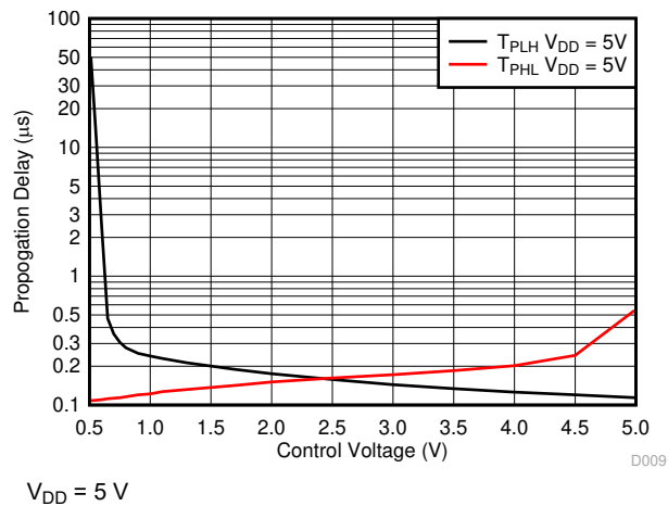
Figure 5-9. Propagation Delay vs Control Voltage
