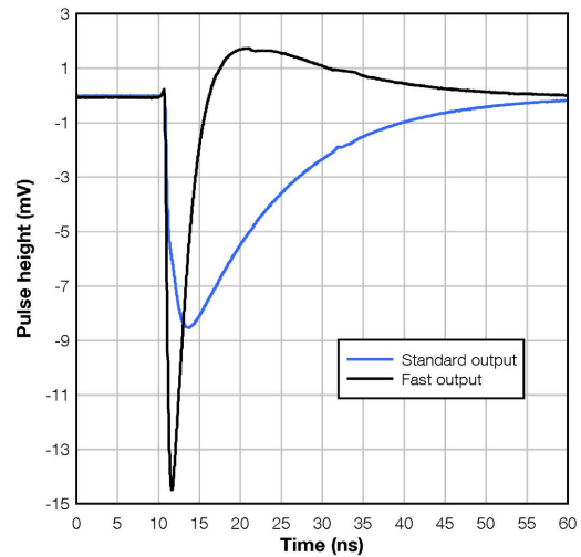
Figure 8. Pulse Shape (MICROB-10010)
