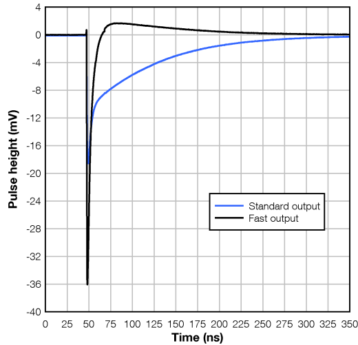
Figure 6. Pulse Shape (MICROB-10035)
