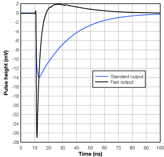
Figure 7. Pulse Shape (MICROB-10020)
