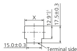
Diagram of recommended for panel mounting holes
