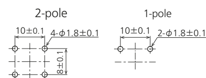
P/C board pattern
