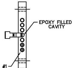
TERMINATION VIEW
