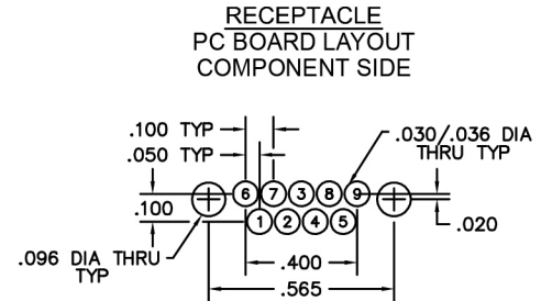
PC BOARD LAYOUT COMPONENT SIDE
