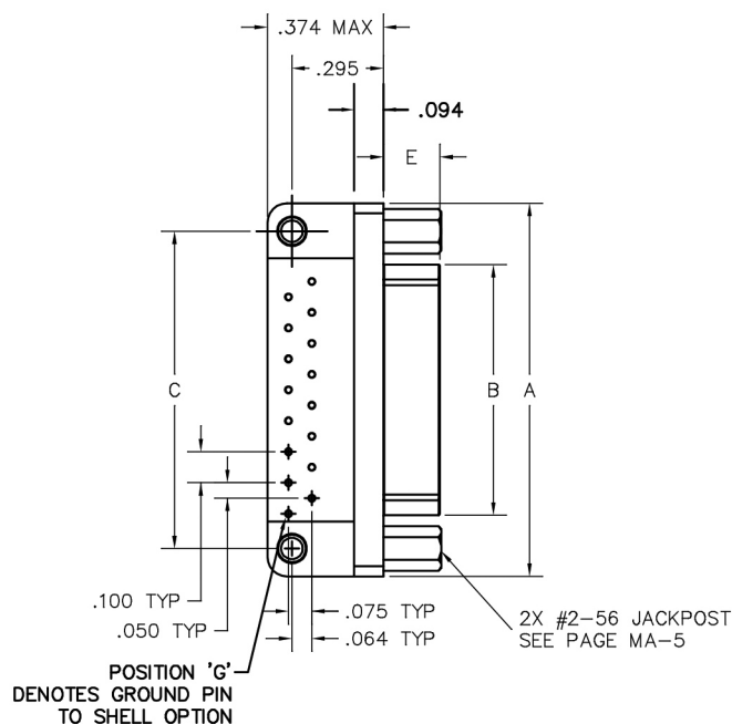
PLUG SHOWN
