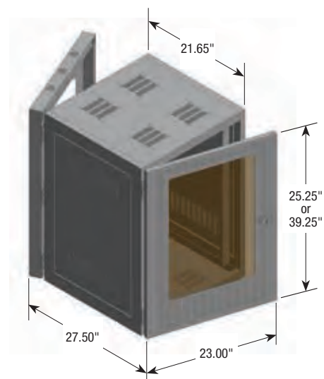
XWM-2312-GD and XWM-2320-GD
