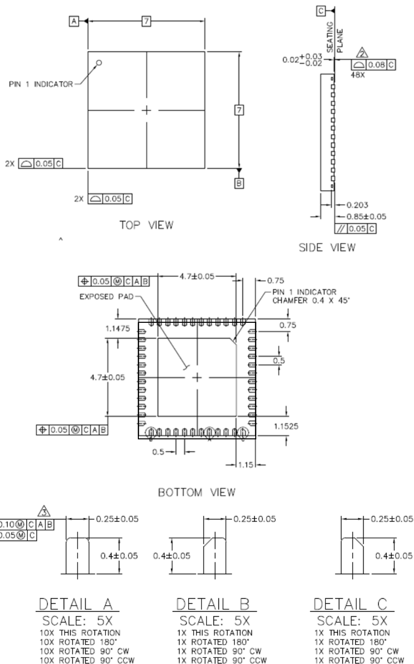
Figure 62. 7x7 mm 48-QFN Package Dimensions
