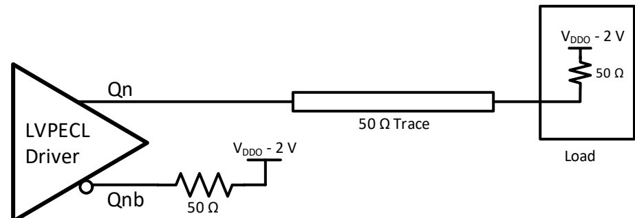
Figure 26. Single-Ended LVPECL Clock Output Termination, DC Coupling
