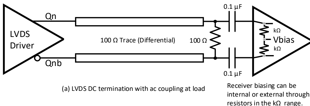
Figure 23. AC-Coupled LVDS Clock Output Coupled to Receivers without Internal 100\ \Omega Termination
