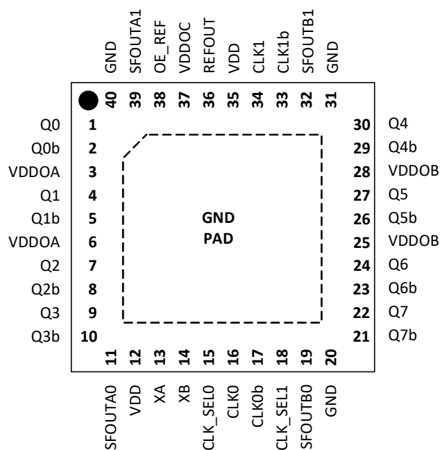
Figure 3. SKY53580 6x6 mm 40-QFN Pinout
