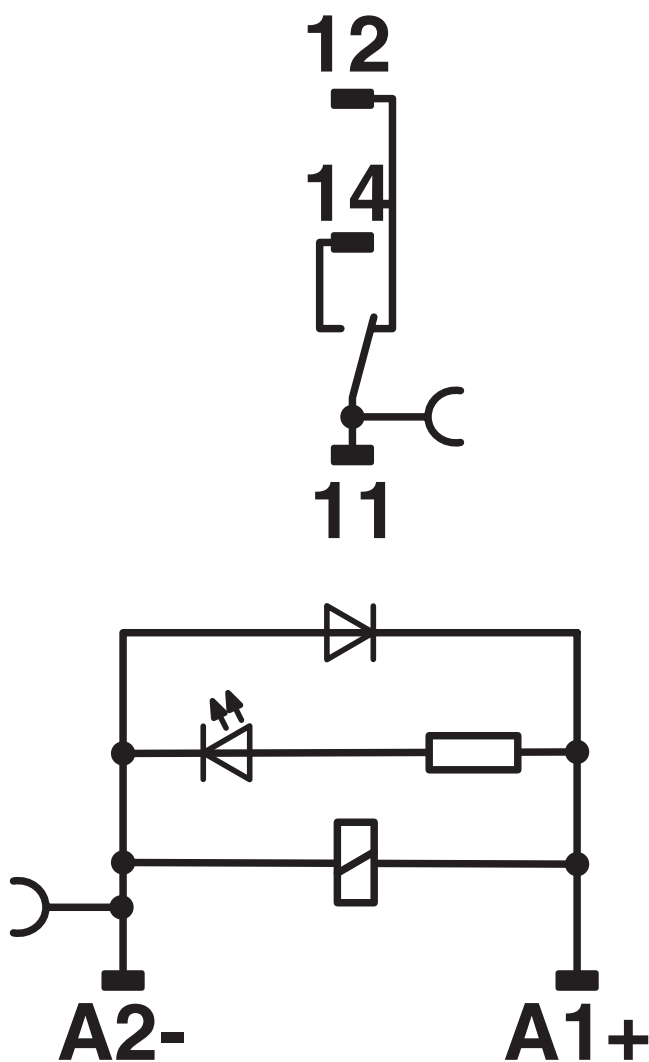
Circuit diagram
