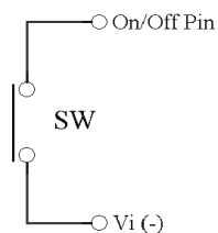
PXD15-xxSxx is turned off with Low-level logic
