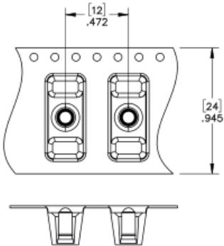
0945-0-57 Tape & Reel Details
