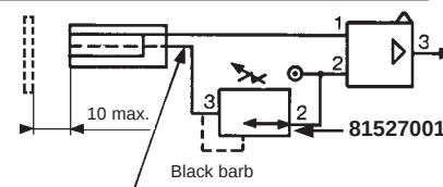
Negative output
