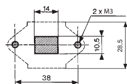
Square lever
