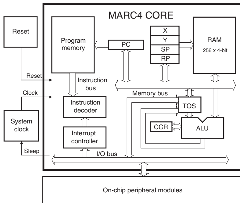
Figure 15-1. Microcontroller Core
