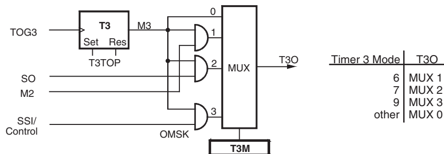
Figure 23-13. Modulator 3
