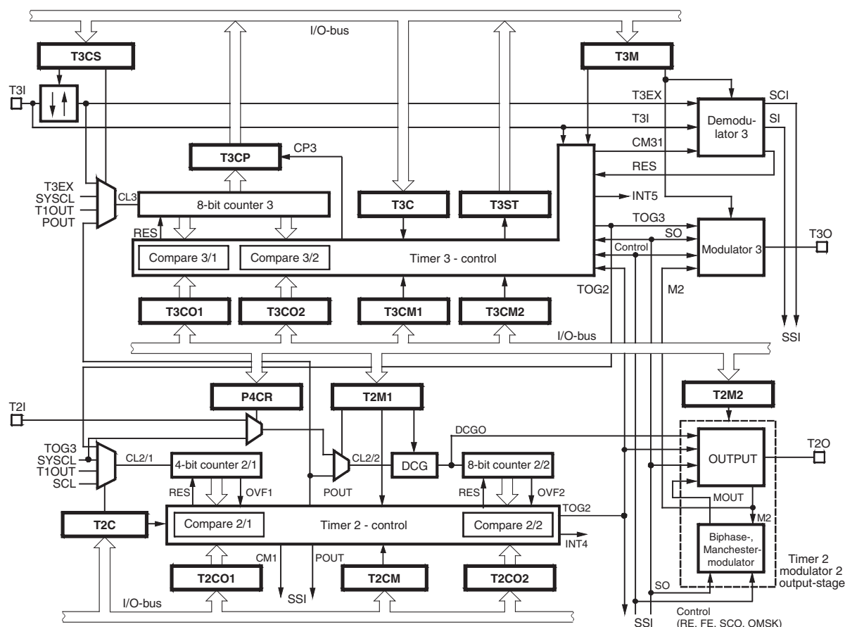
Figure 24-12. Combination Timer 3 and Timer 2
