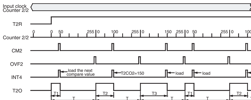
Figure 22-22. PWM Modulation
