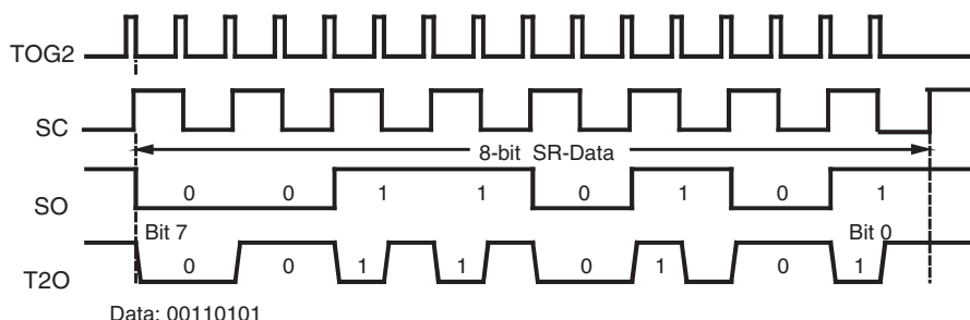
Figure 22-20. Biphase Modulation
