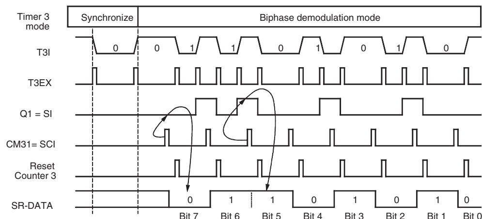
Figure 23-11. Biphase Demodulation
