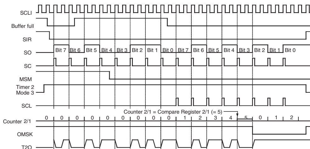
Figure 24-6. Biphase Modulation 2
