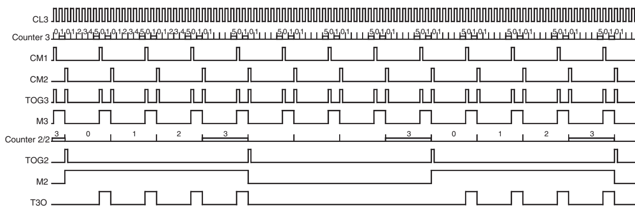
Figure 24-15. Burst Modulation 1
