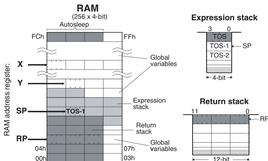
Figure 16-2. RAM Map
