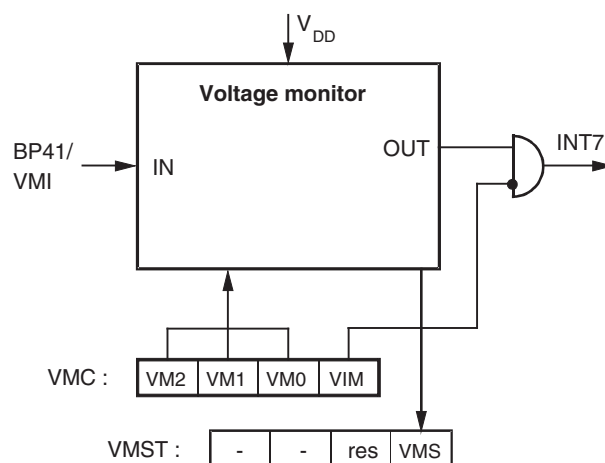
Figure 18-1. Voltage Monitor
