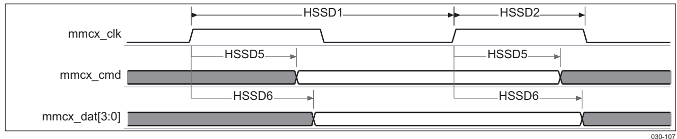
Figure 6-66. MMC/SD/SDIO – High-Speed SD Mode – Data/Command Transmit
