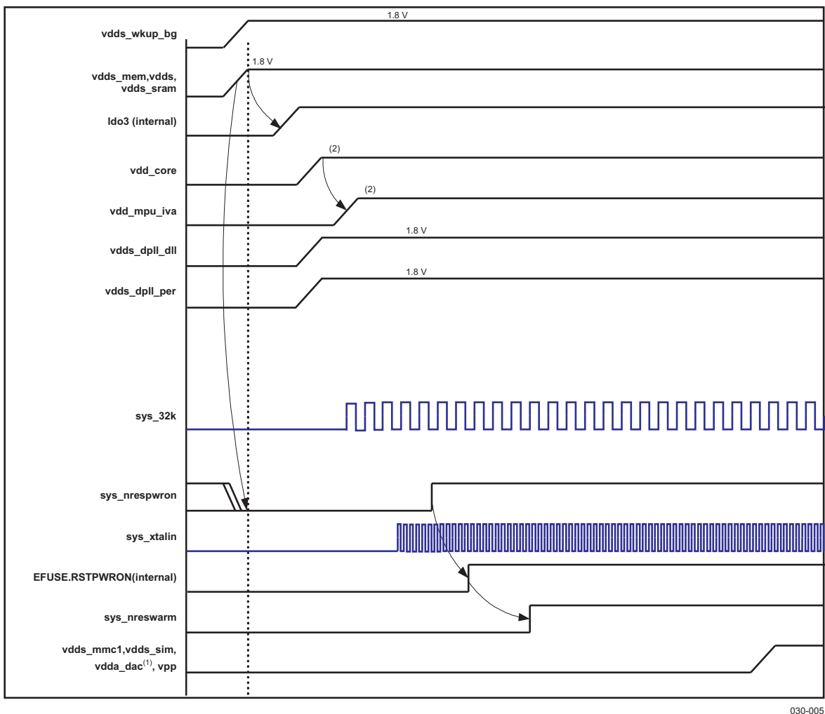
Figure 3-3. Power-up Sequence
