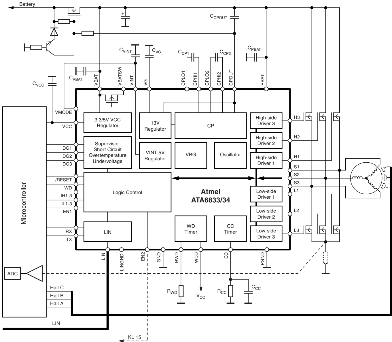
Figure 9-1. Typical Application
